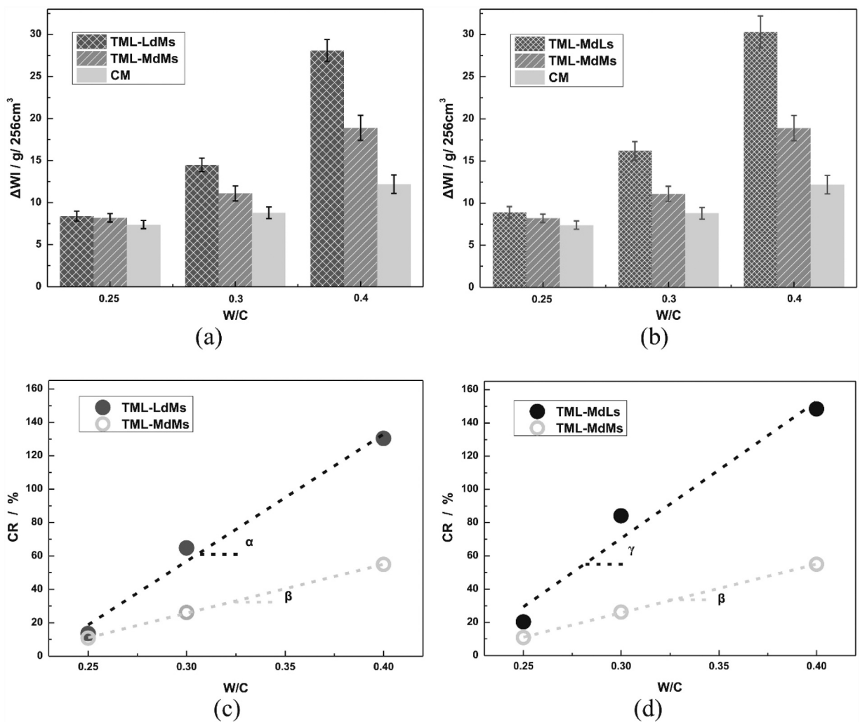
Fig. 11. Carbon capture ability results (a) Weight increase of samples (TML-LdMs, TML-MdMs, and CM); (b) Weight increase of samples (TML-MdLs, TML-MdMs, and CM); (c) The relationship of CR against W/C for TML-LdMs and TML-MdMs; and (d) The relationship of CR against W/C for TML-MdLs and TML-MdMs. Liu et al., [90].
